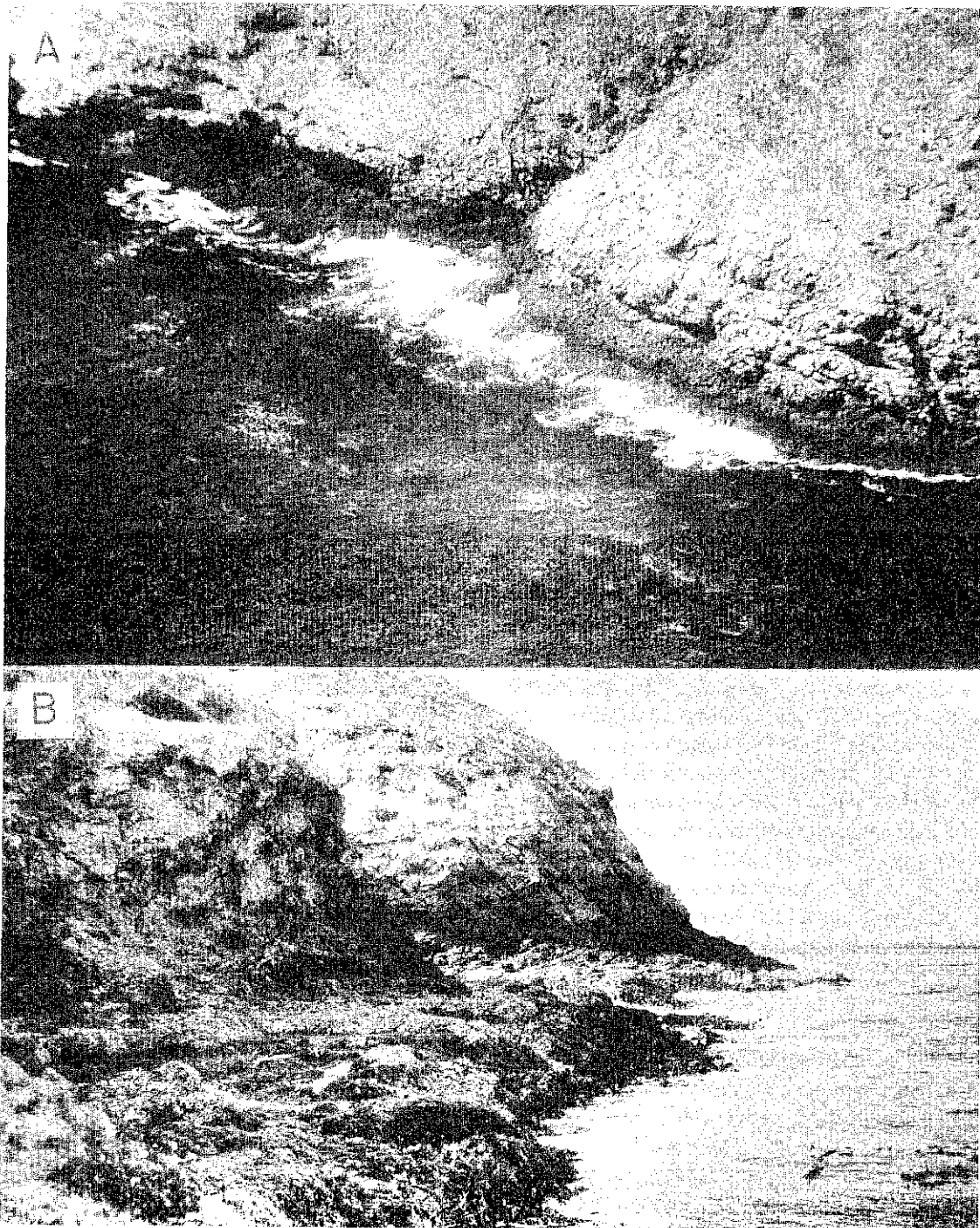
Figure 2. (A) Aerial photograph of study area on Santa Barbara Island. The diagonal indentation in the cliffs (upper center of photograph) marks Cave Canyon. (B) Northward view of shoreline at study site. Steep bluffs are located immediately shoreward of the narrow intertidal bench. The mouth of Cave Canyon is situated between the two bluffs.
