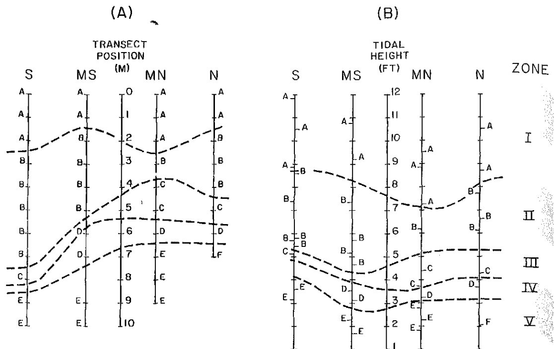
Figure 4. Location of quadrats comprising cluster groups identified in Figure 3: A) along transect lines as a function of distance downshore (in meters) and B) along transect lines repositioned according to tidal heights. Dashed lines have been added to separate cluster groups and to define vertical zones on the shore.
