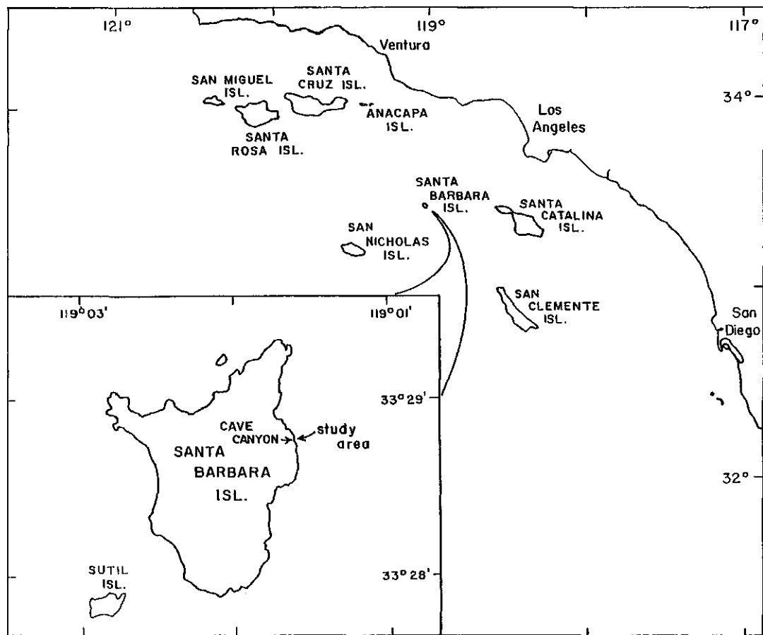
Figure 1. Location of Santa Barbara Island in the Southern California Bight and (inset) study area at Cave Canyon, Santa Barbara Island.
