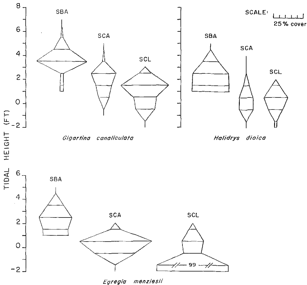
Figure 7. Comparisons of the vertical distributions (as kite diagrams of percent cover) for three species of macrophytes at Santa Barbara Island (SBA) in November 1975, Santa Catalina Island (SCA) in November 1975 and San Clemente Island (SCL) in December 1975. Mean abundance data for each 1-ft tidal interval for Santa Catalina and San Clemente Islands from Littler (1977).
