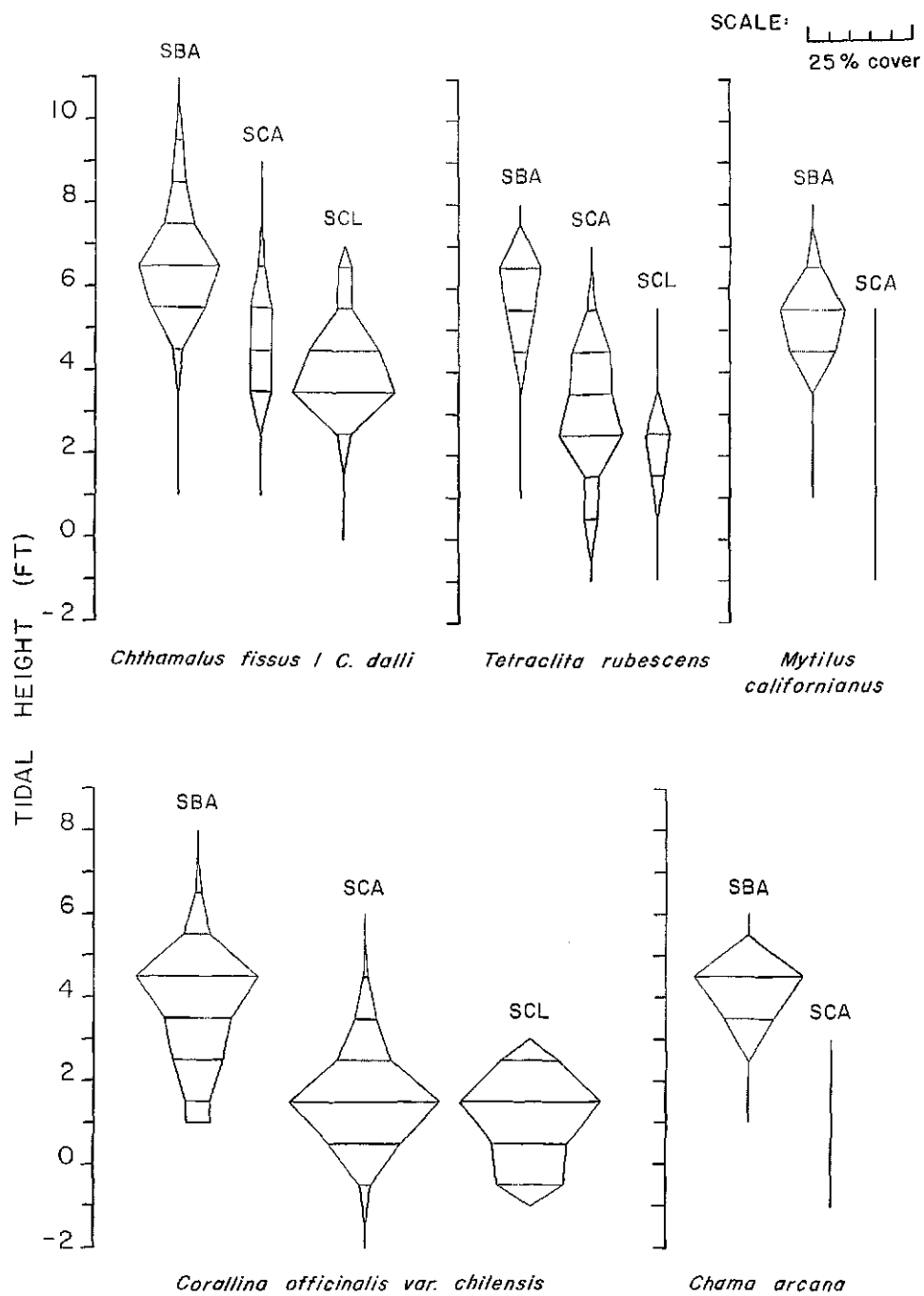
Figure 6. Comparisons of vertical distributions (as kite diagrams of percent cover) for four species of invertebrates and one species of macrophyte sampled at Cave Canyon, Santa Barbara Island (SBA) in November 1975, Big Fisherman's Cove, Santa Catalina Island (SCA) in November 1975 and Wilson Cove, San Clemente Island (SCL) in December 1975. Mean abundance data for each 1-ft tidal interval for Santa Catalina and San Clemente Islands from Littler (1977).
