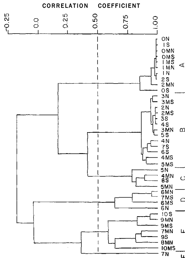
Figure 3. Cluster analysis dendrogram for all quadrats sampled in November 1975 at Cave Canyon, Santa Barbara Island. Quadrats are coded by number (meters downshore on each transect line, with 0 at top of line) and either N, MN, MS, or S (referring to North, Middle North, Middle South or South transect lines).
