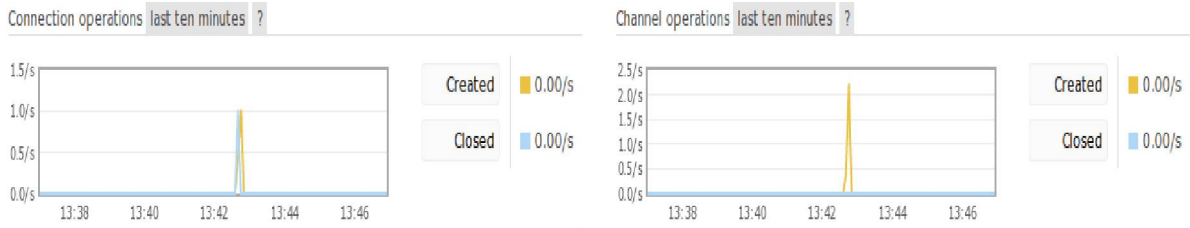
Figure 5.7: churn rate
