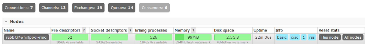
Figure 5.4: RMQ node
