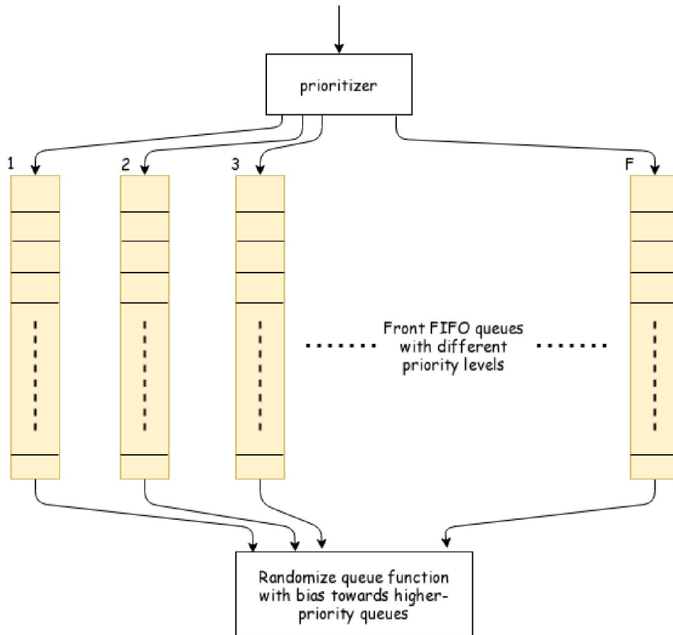
Figure 2.5: Frontier Front Queue [12]
