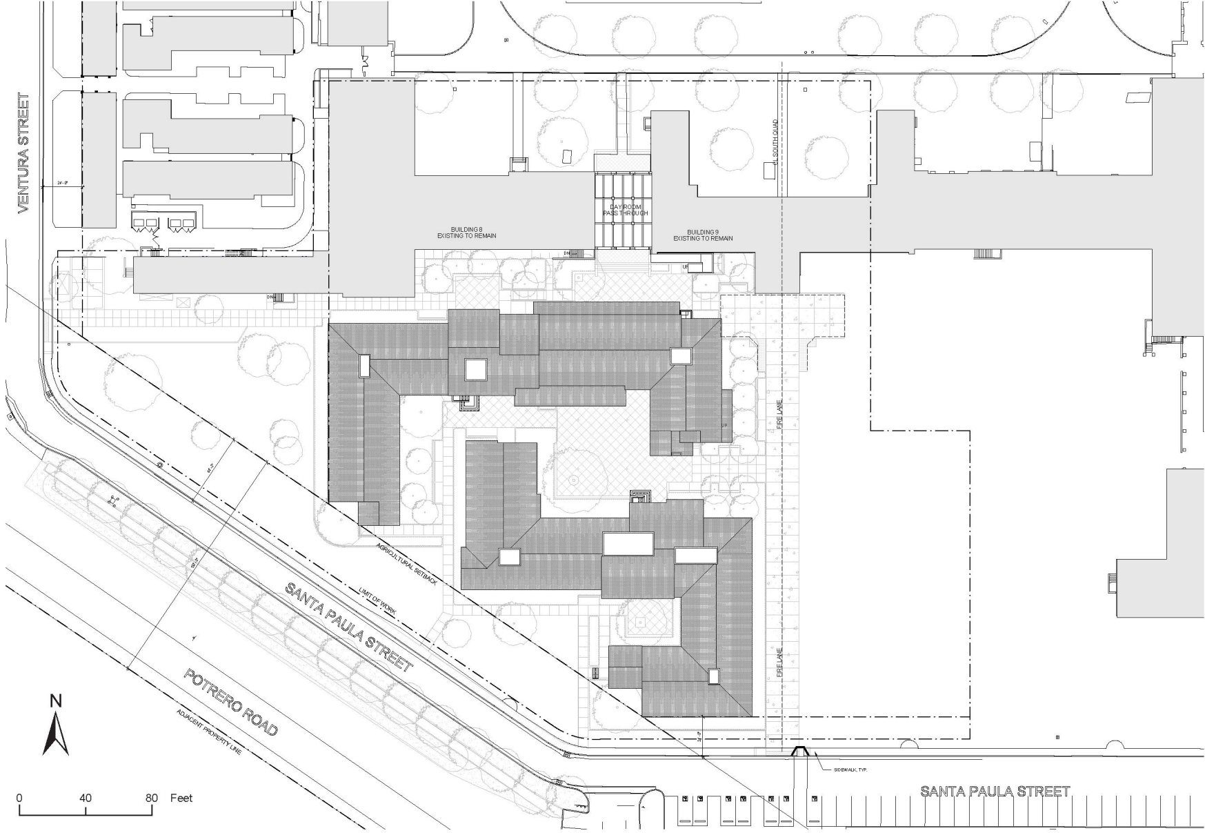
Site Plan
